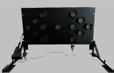
Truck mounted Standard frame + LINKA actuator
